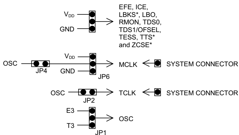
Figure 2. DS3150DK JUMPERS
